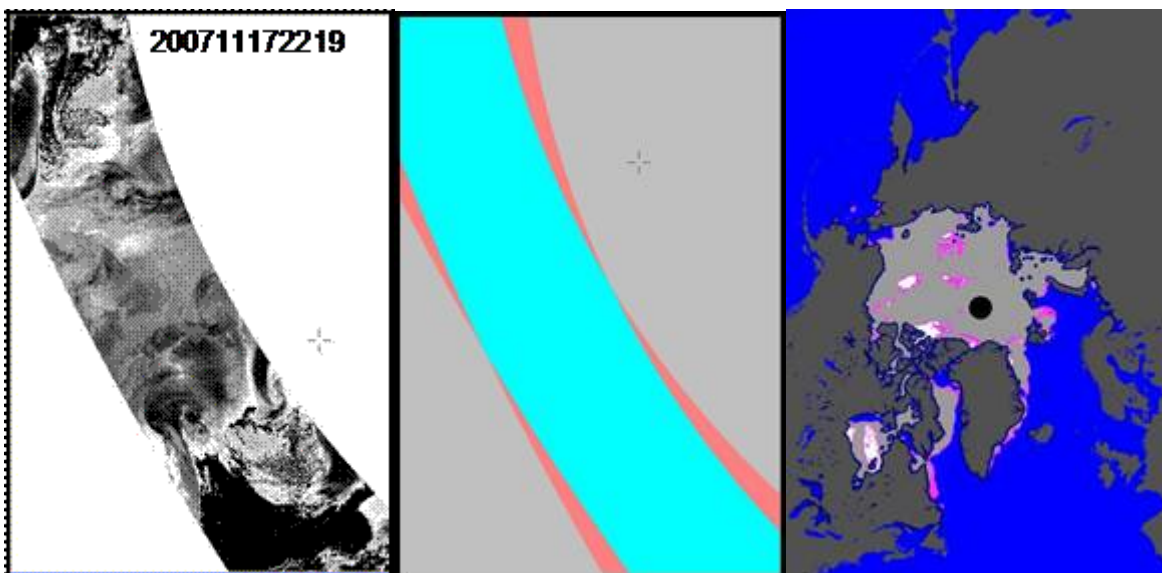
Figure 4 Left is an IR swath transformed into the 1 km grid of OSI SAF NH area. In the middle is the overlap between two swath separated by 24h show in blue, and right in an example of the OSI SAF ice type product.
